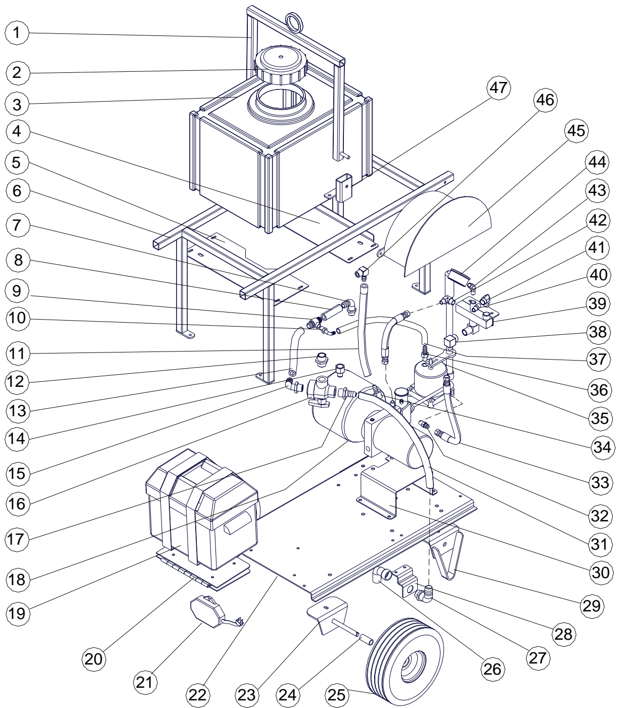
SHORELOCK PUMP, ELECTRIC PARTS BREAKDOWN
